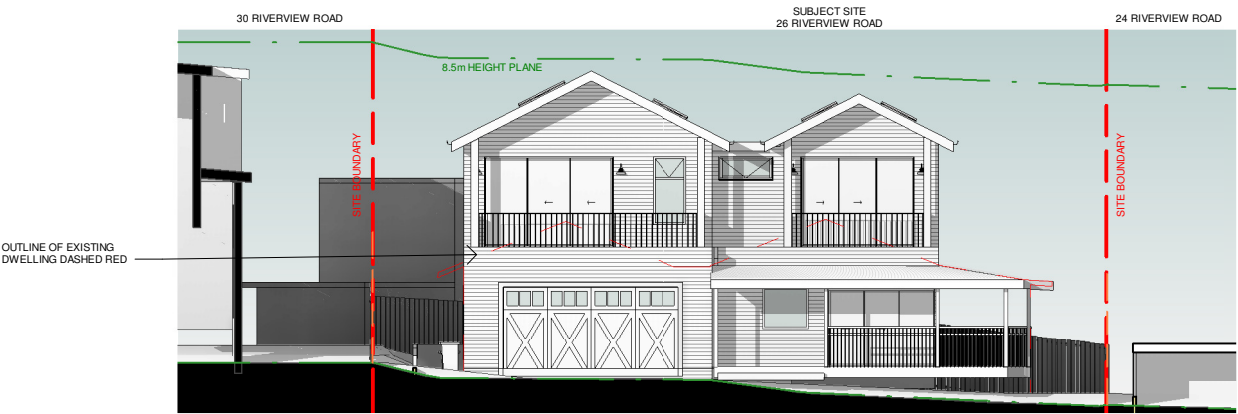
NN WEST ELEVATION - REAR HOUSE SCALE: 1 : 200
