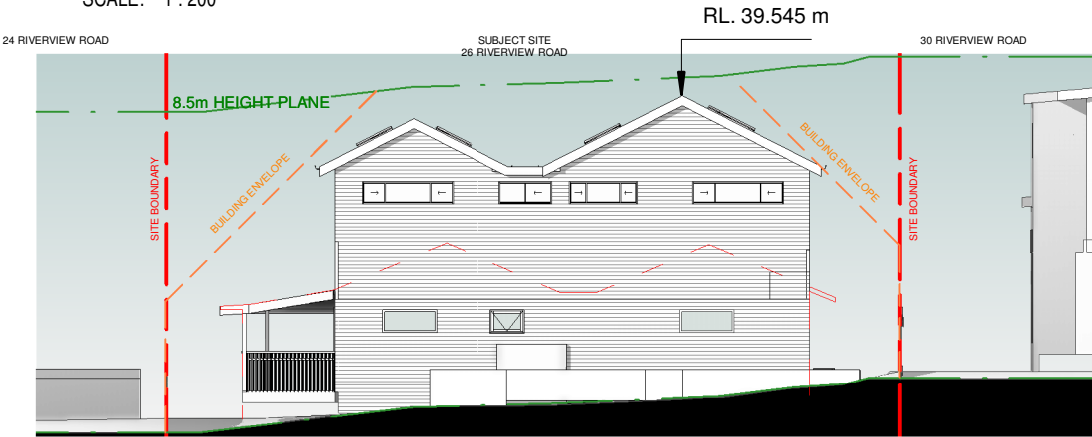
NN NORTH ELEVATION - REAR HOUSE SCALE: 1 : 200
