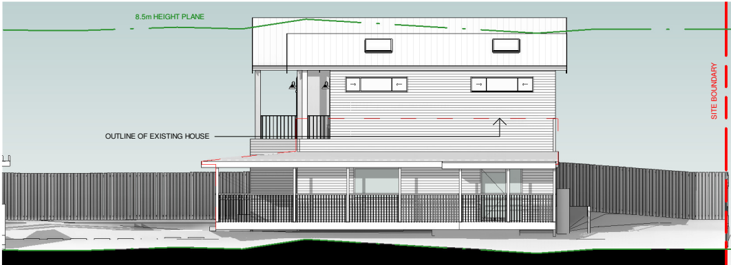
NN SOUTH ELEVATION - REAR HOUSE SCALE: 1 : 200
