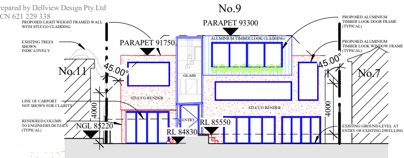
PROPOSED NORTH ELEVATION (DWELLING)
