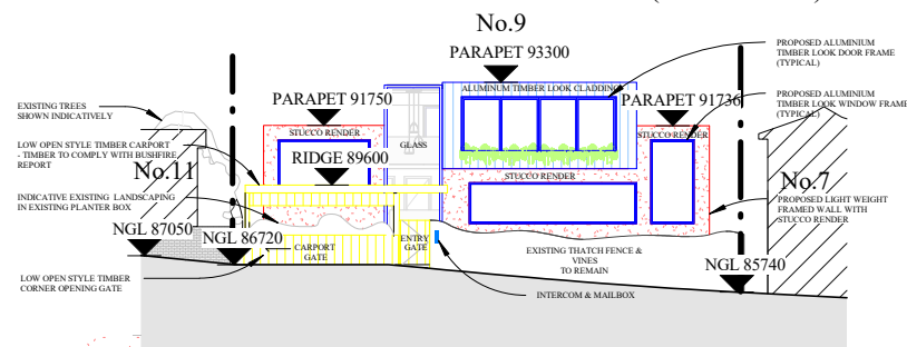
PROPOSED NORTH ELEVATION (STREET VIEW)
