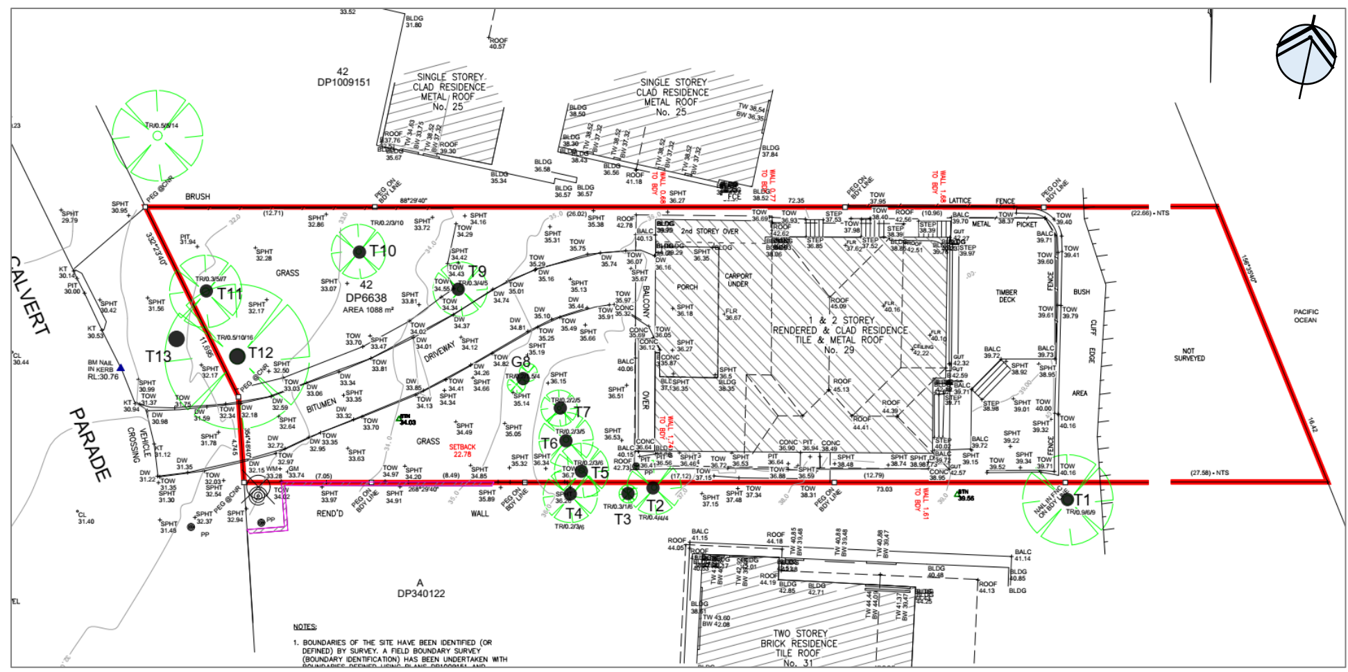
Figure 1 - Marked Up Survey Plan - Dwg no. 1978TN, dated 06/02/2024 authored by True North Surveys. NOT TO SCALE.
