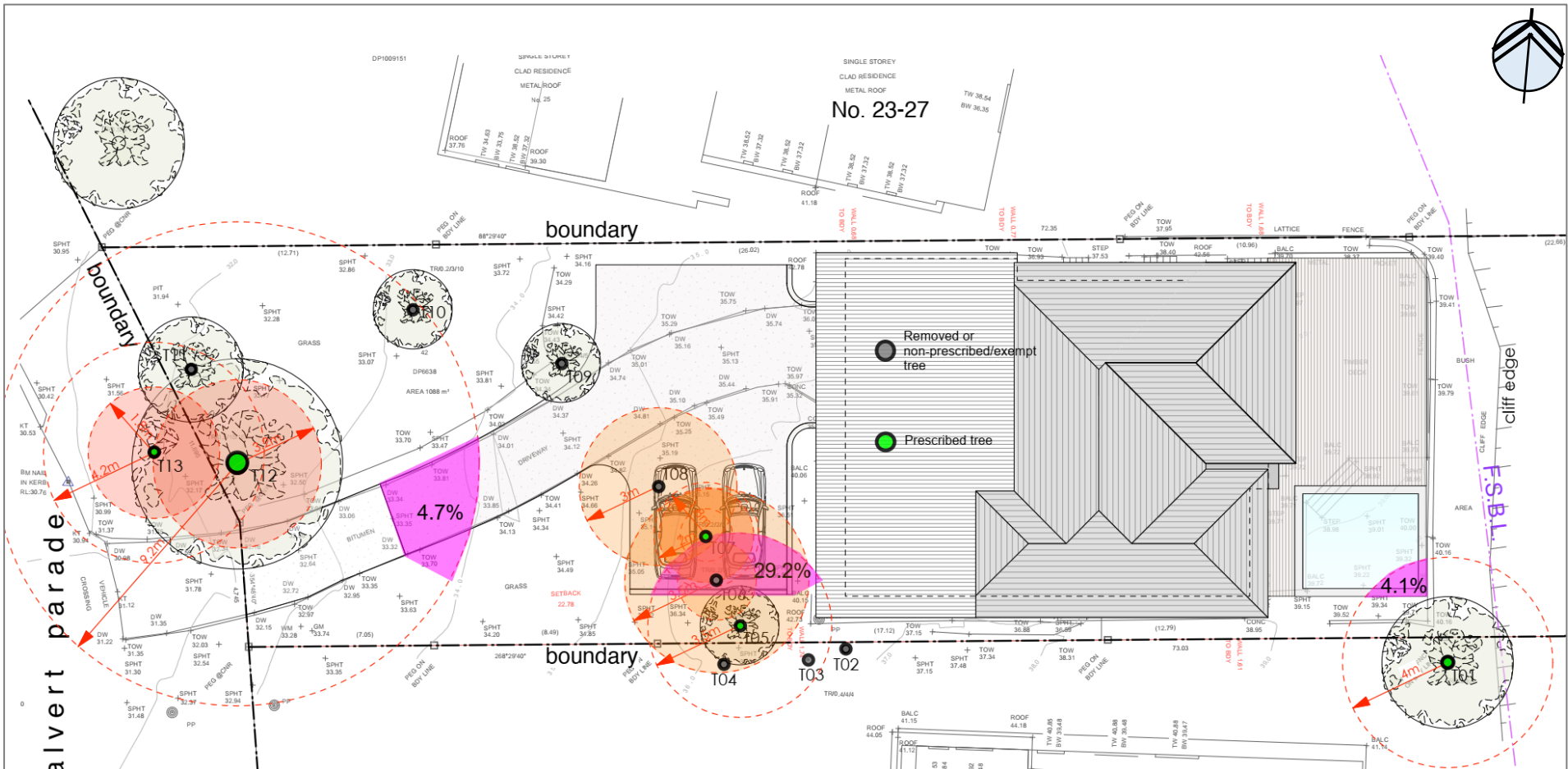
Figure 2 - Marked Up Tree Zones Plan, dwg no. A17, dated September 2024 authored by Andy Lehman Design. Orange shaded circle tree proposed for removal, Red hashed circle TPZ calculation, red shaded inner circle SRZ calculation, pink shading estimated encroachment. Prescribed/non-prescribed tree as indicated. Marked up by C Hughes. NOT TO SCALE.
