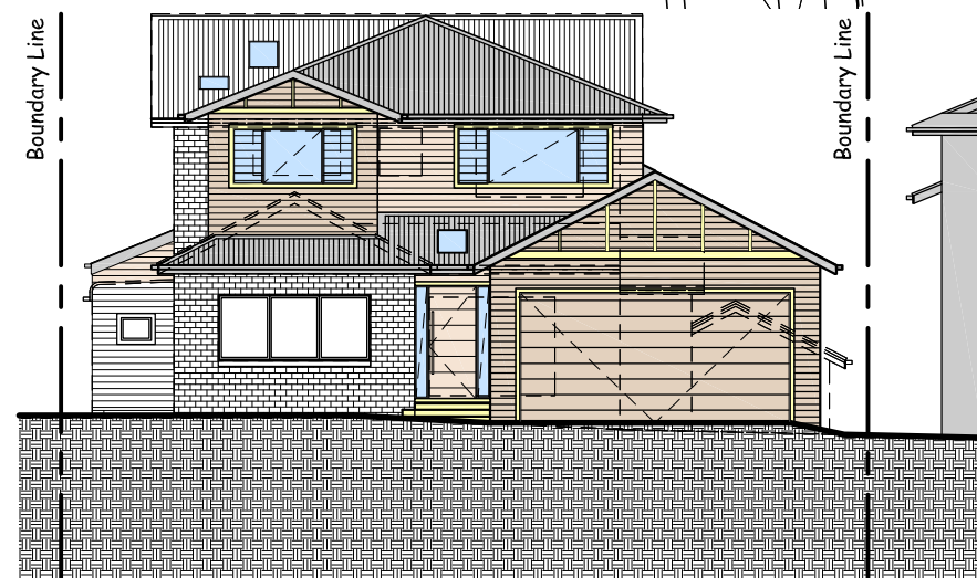
Elevation South
