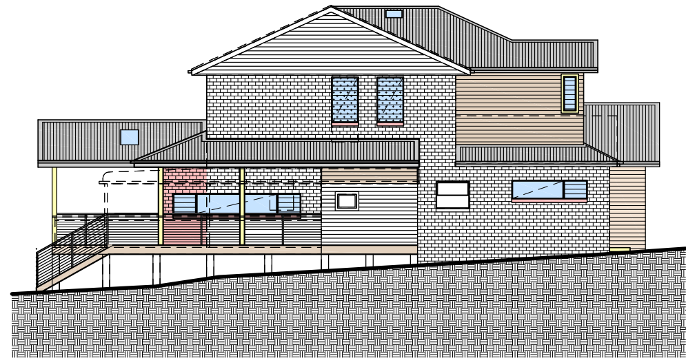
Elevation West
