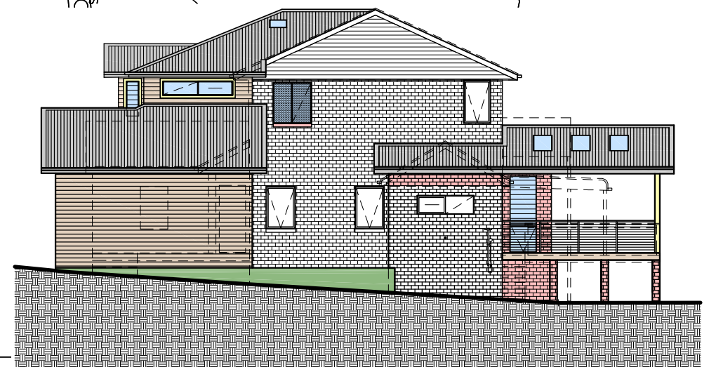
Elevation East
