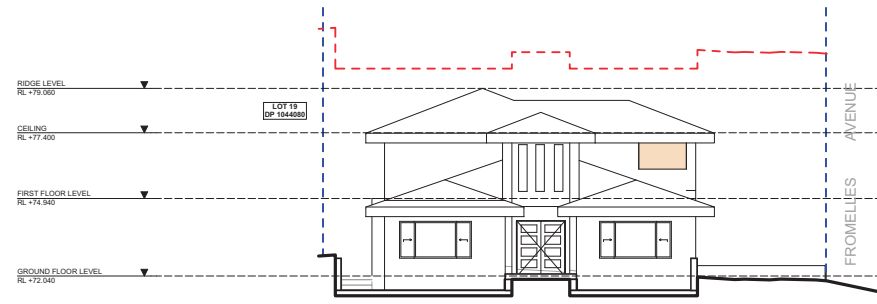
3 SOUTH ELEVATION 1:200
