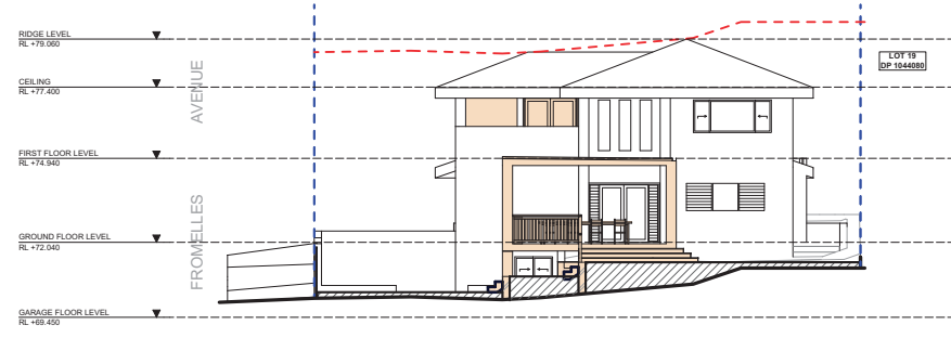
2 NORTH ELEVATION 1:200
