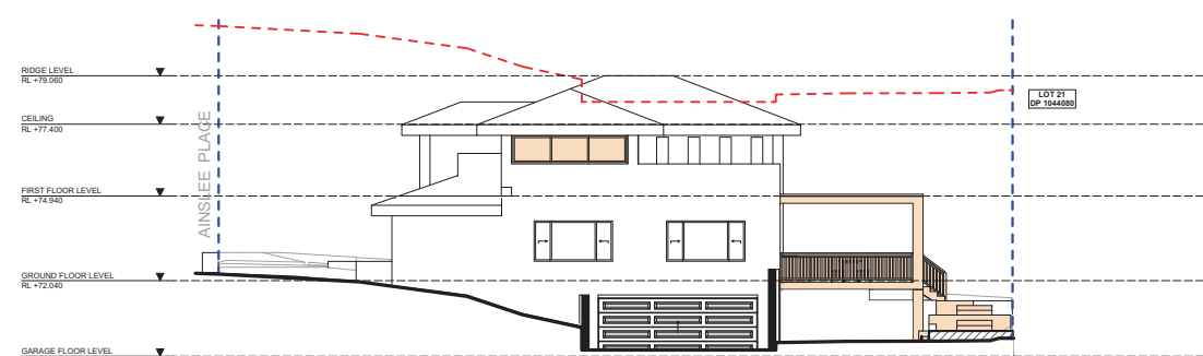
5 EAST ELEVATION 1:200
