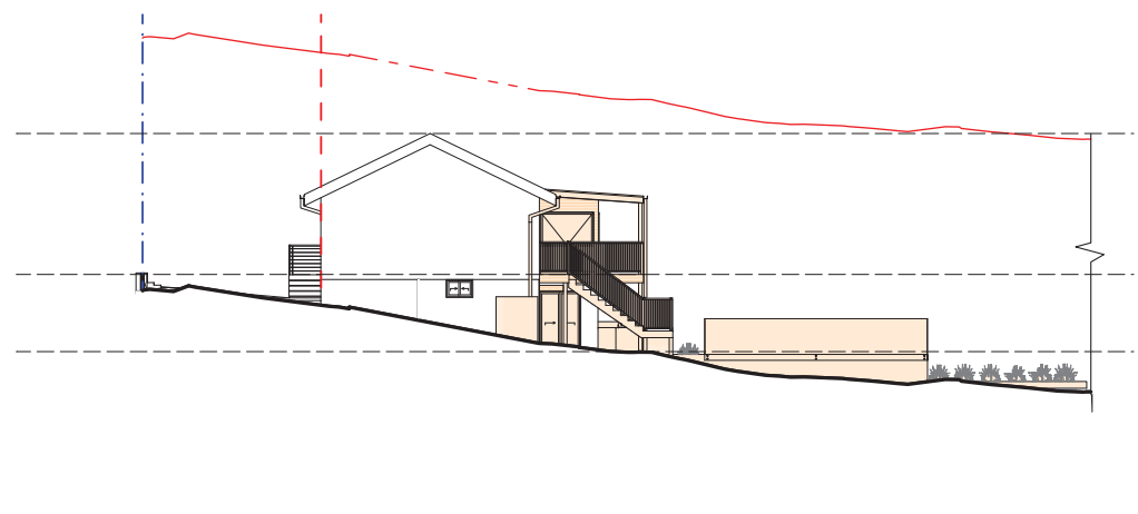
5 NORTH ELEVATION 1:200
