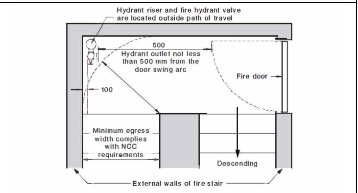
Figure H.3(C) — Internal fire hydrant clearances required within a fire isolated stair
