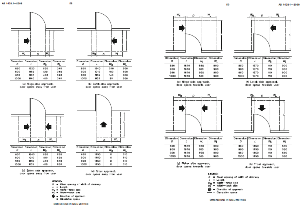
FIGURE 31 (in part) CIRCULATION SPACES AT DOORWAYS WITH SWINGING DOORS
