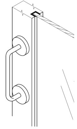
ISOMETRIC VIEW
