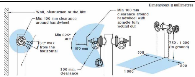
Figure H.3(A) — External fire hydrant clearances
