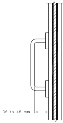
SECTIONAL ELEVATION
