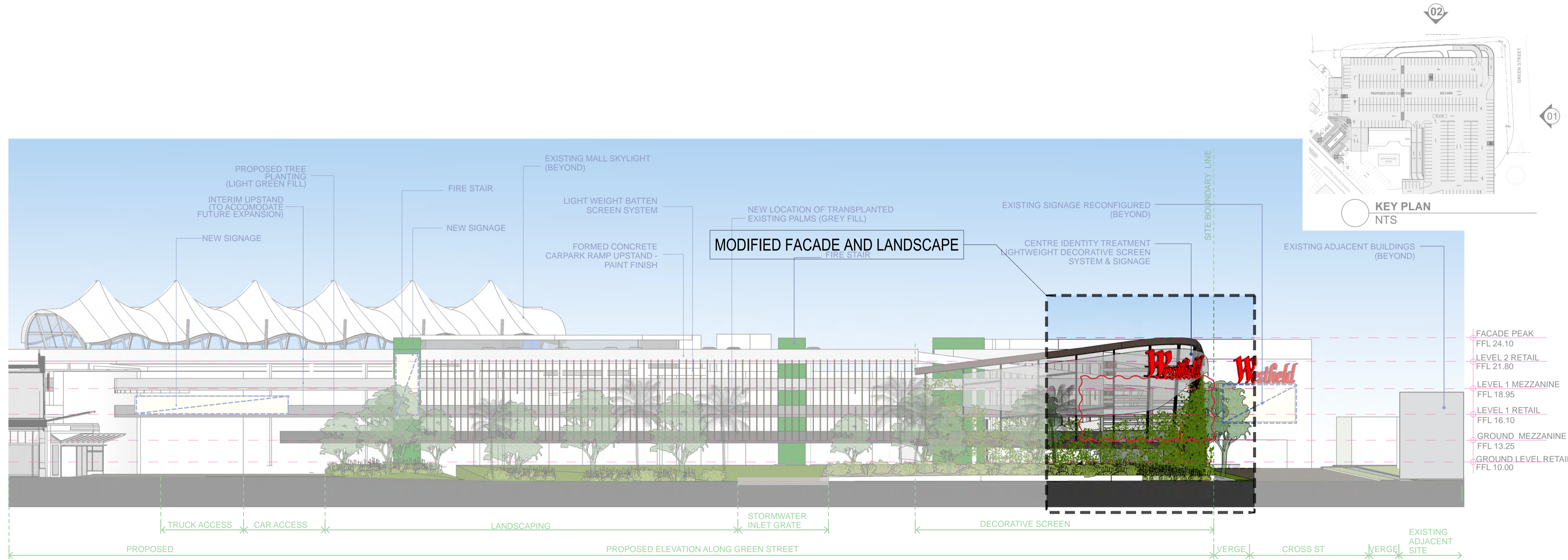
01 EAST ELEVATION - GREEN STREET 1:250
