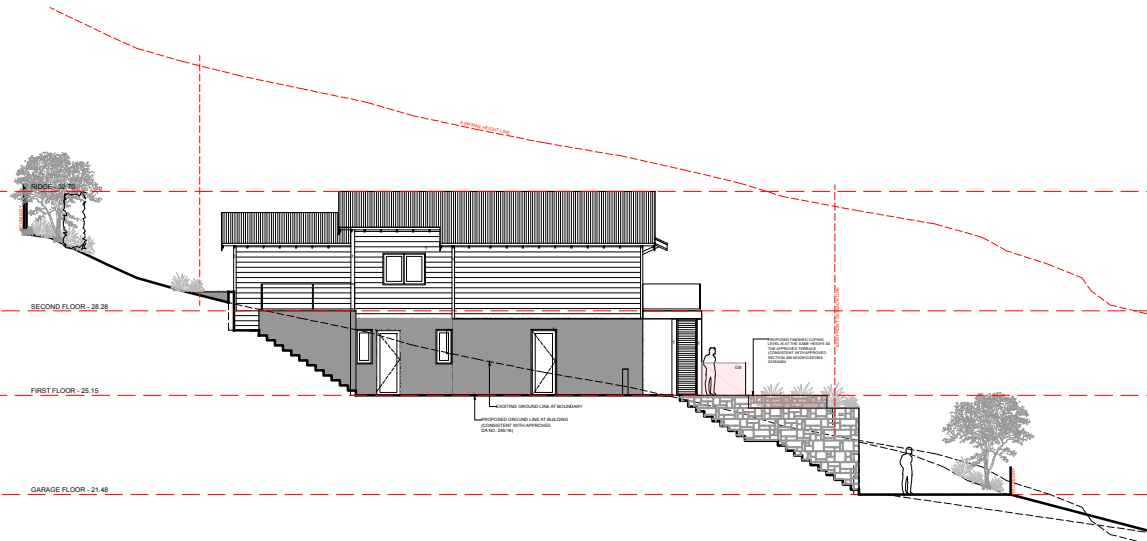
EAST ELEVATION
