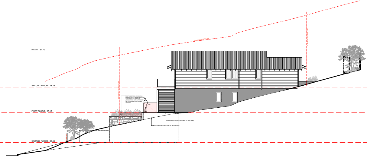
WEST ELEVATION
