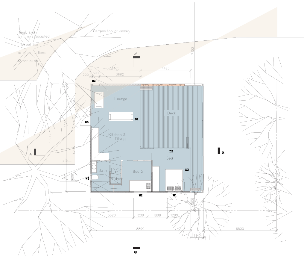
FLOOR PLAN
