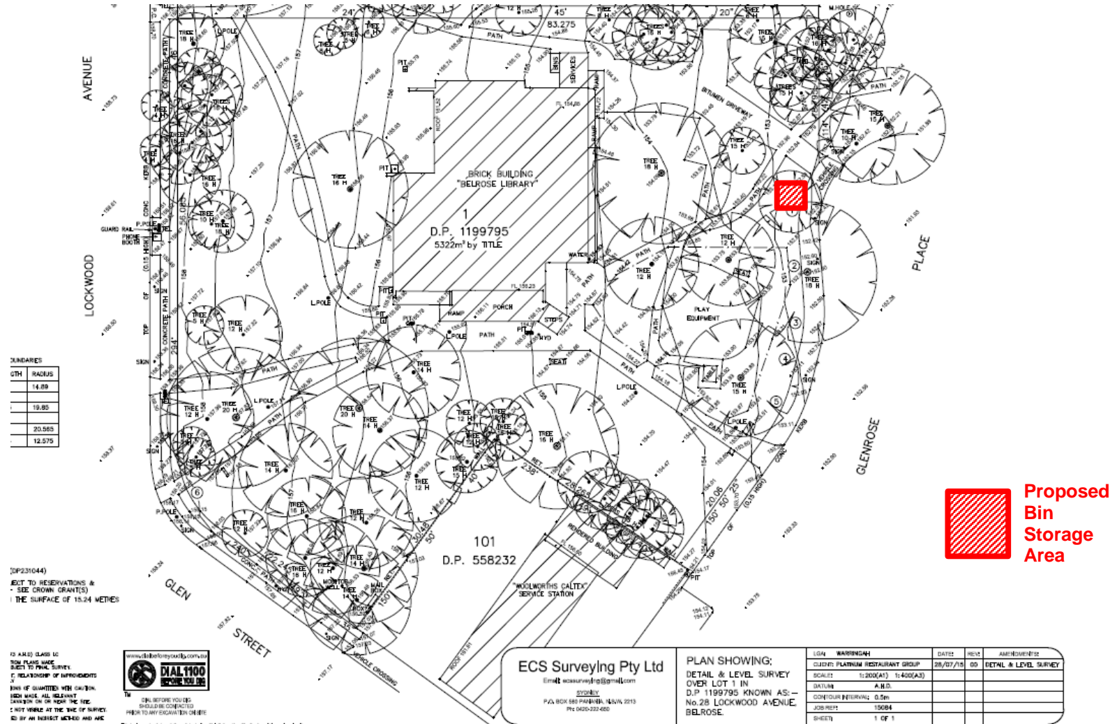
Source: ECS Surveying Pty Ltd, 28 Lockwood Ave Belrose – Detail & Level Survey
