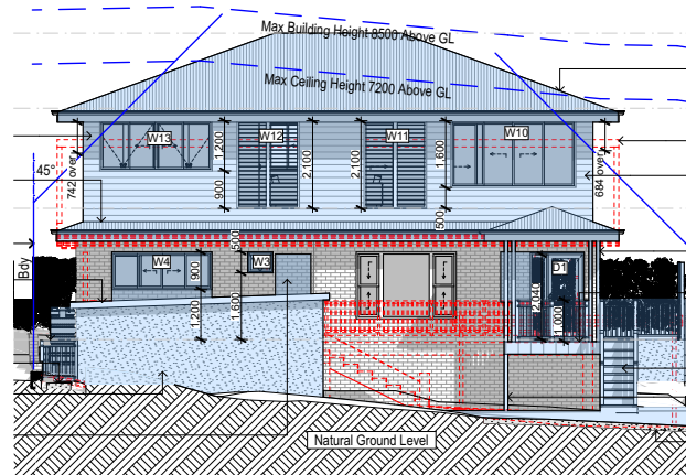
East 1:200
