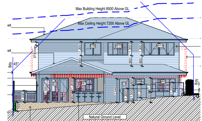
West 1:200
