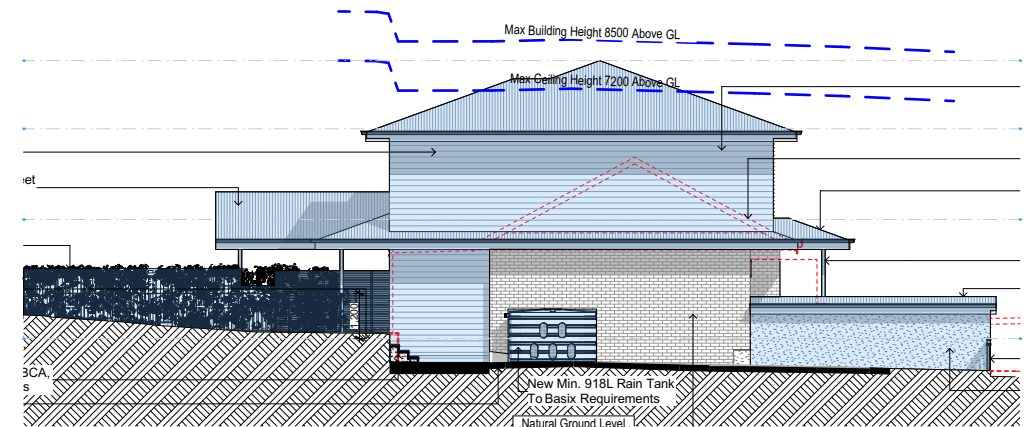
South 1:200
