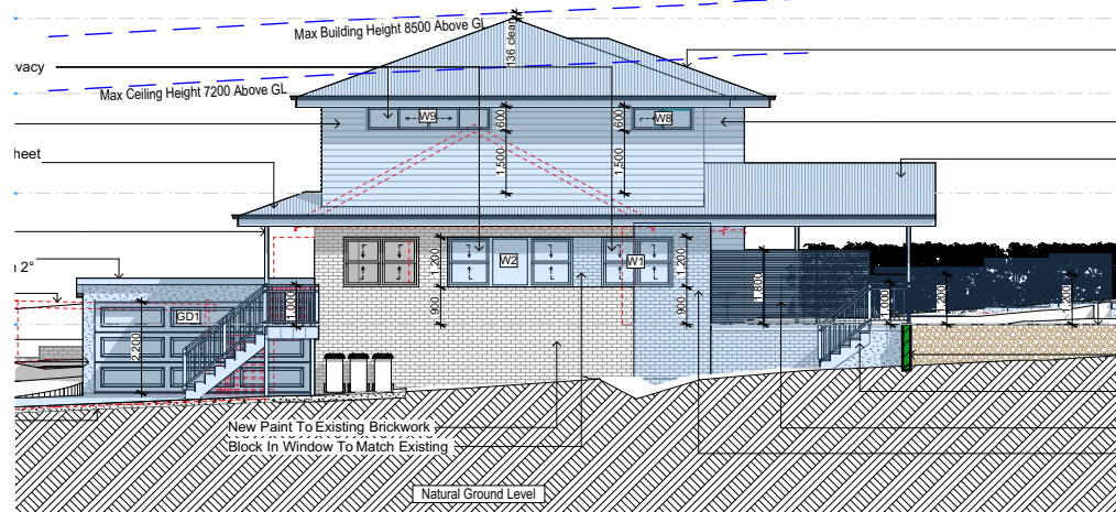
North 1:200
