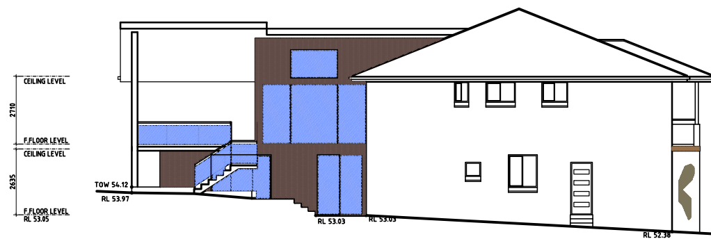
NORTH WEST ELEVATION SCALE 1:100
