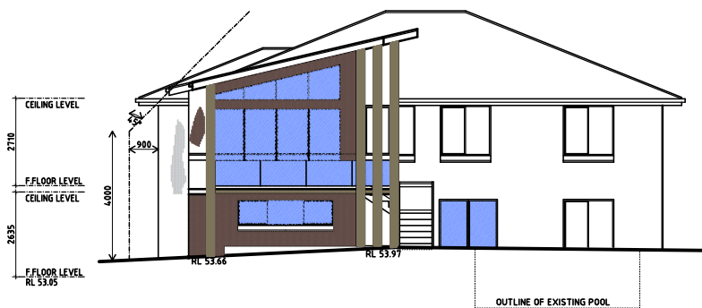
NORTH EAST ELEVATION SCALE 1:100
