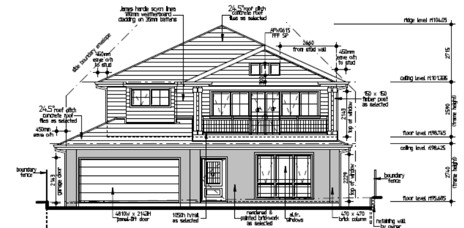
EAST ELEVATION 1:100
