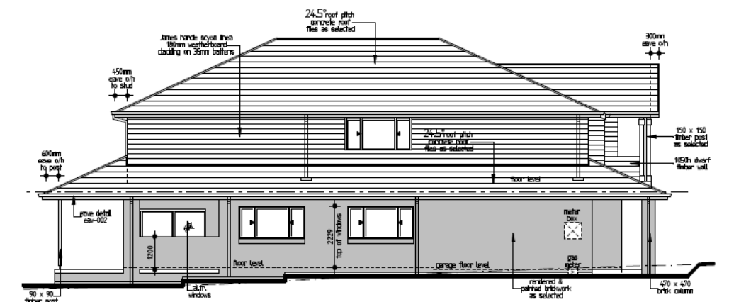
SOUTH ELEVATION 1:100
