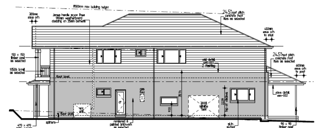
NORTH ELEVATION 1:100
