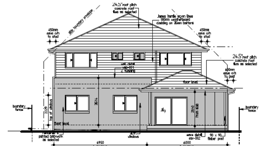
WEST ELEVATION 1:100
