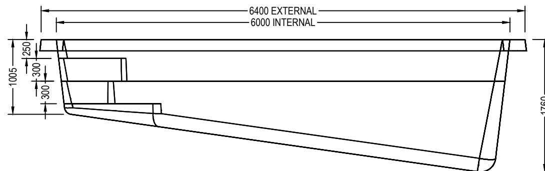
SIDE ELEVATION
