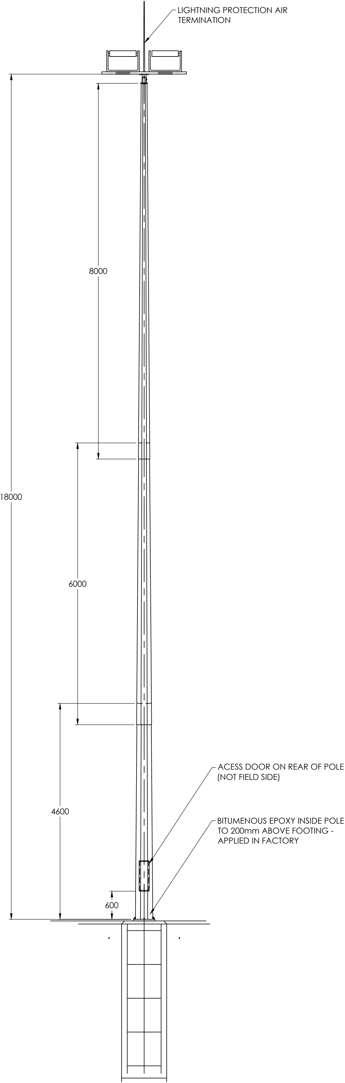
02 SPORTS FIELD LIGHT POLE - FRONT ELEVATION SCALE 1:50@A1
