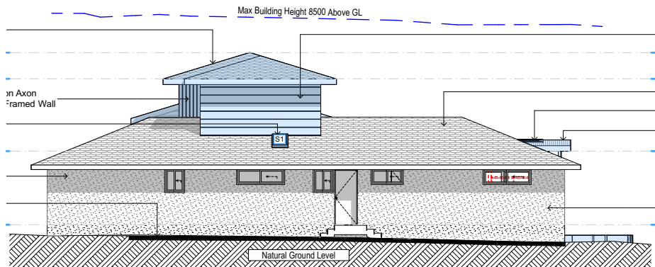
South 1:200
