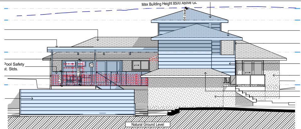
North 1:200
