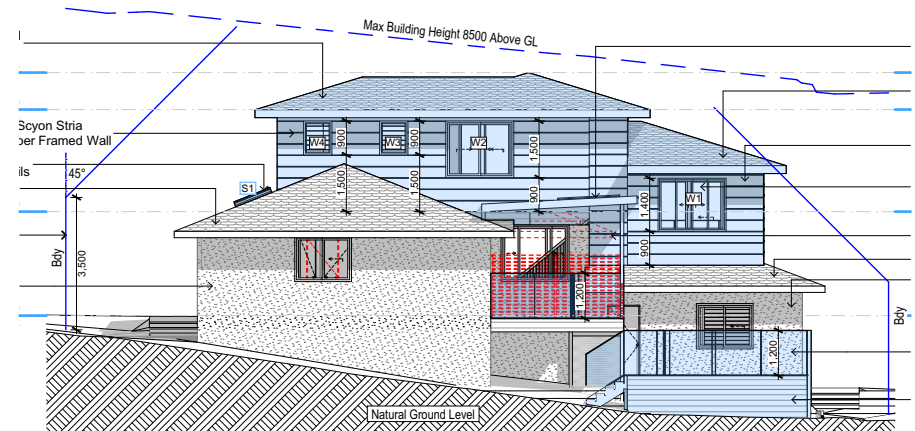
East 1:200
