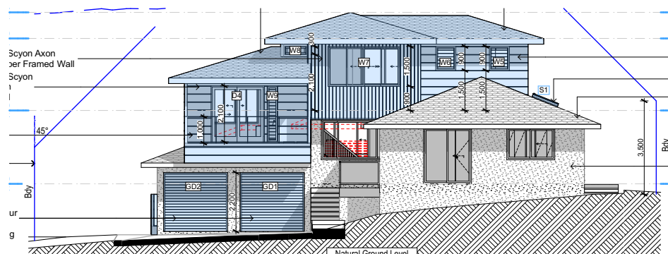
West 1:200
