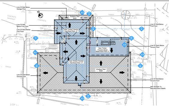
Roof Plan 1:500
