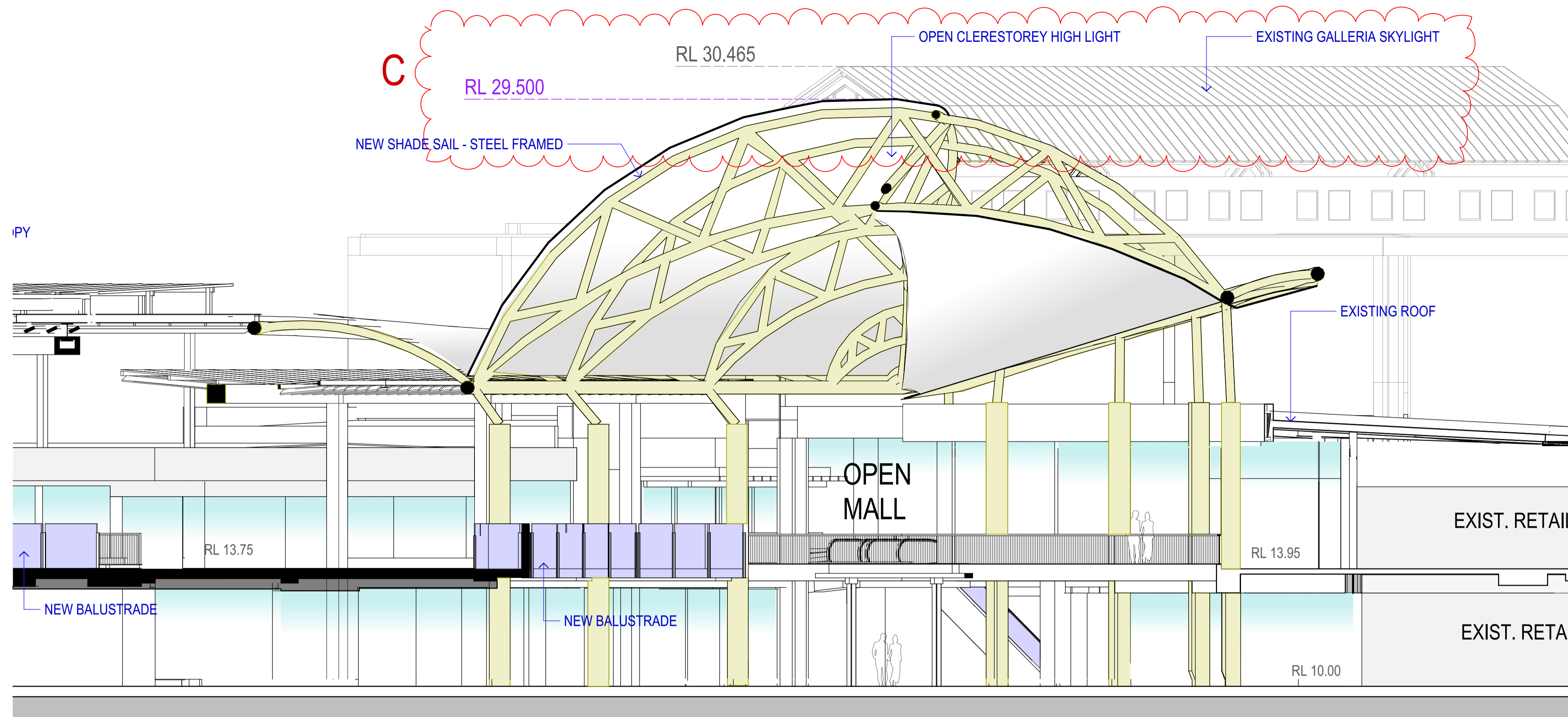
1 SECTION E: SHORT - Looking NW 1:100
