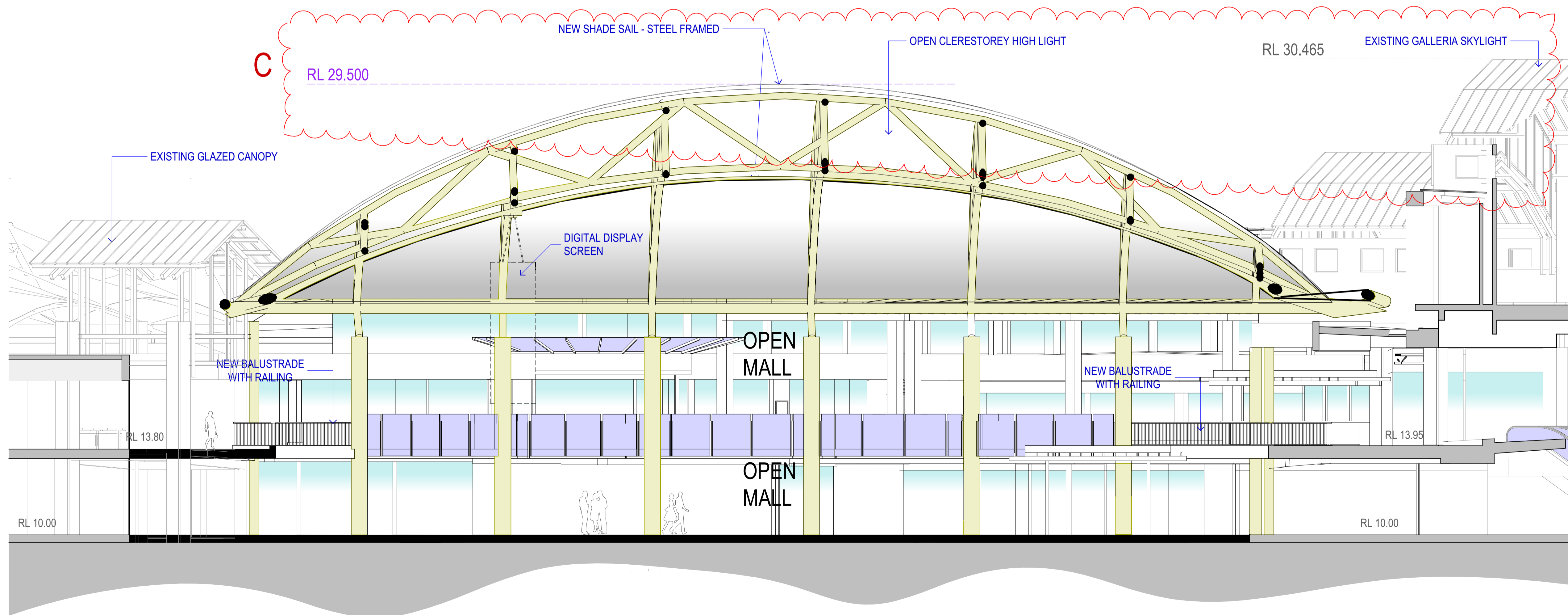
2 SECTION F: LONG - Looking SW 1:100
