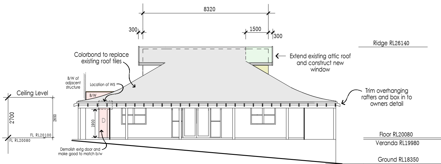
North Elevation
