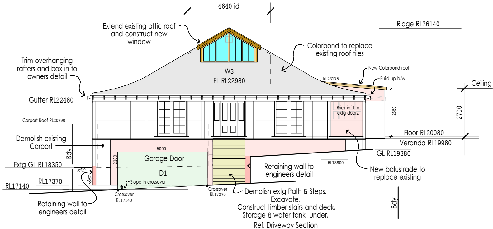
West Elevation
