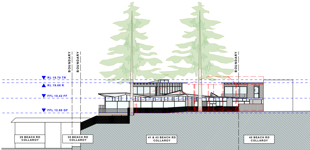
02 EAST ELEVATION PROPOSED 1/500 @ A4
