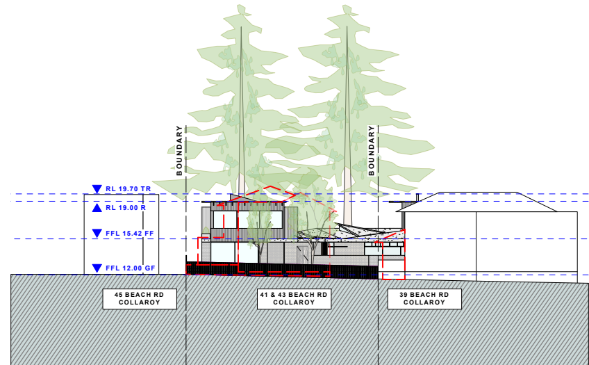
04 WEST ELEVATION PROPOSED 1/500 @ A4
