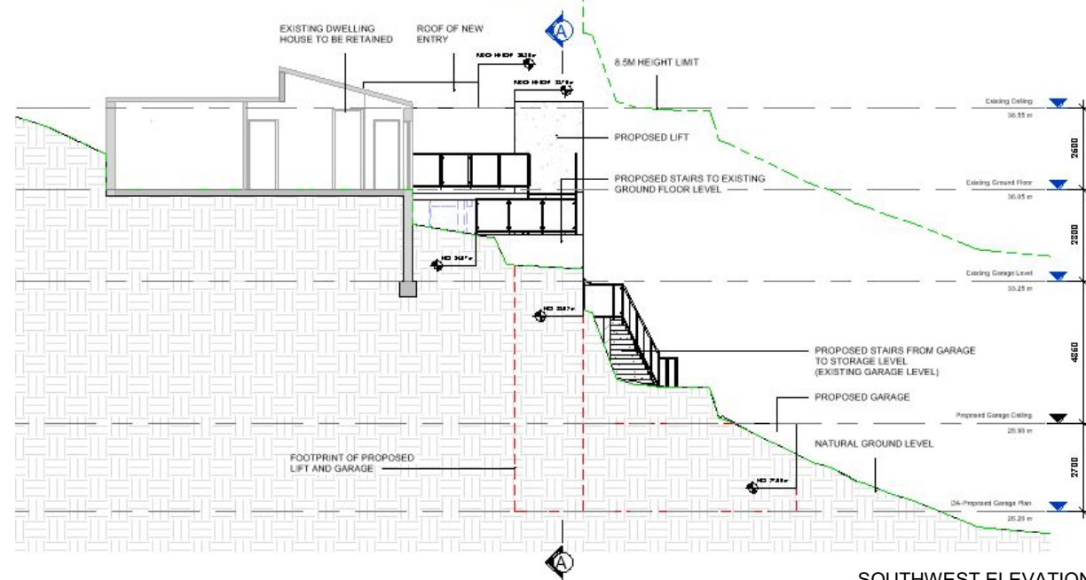
SOUTHWEST ELEVATION
