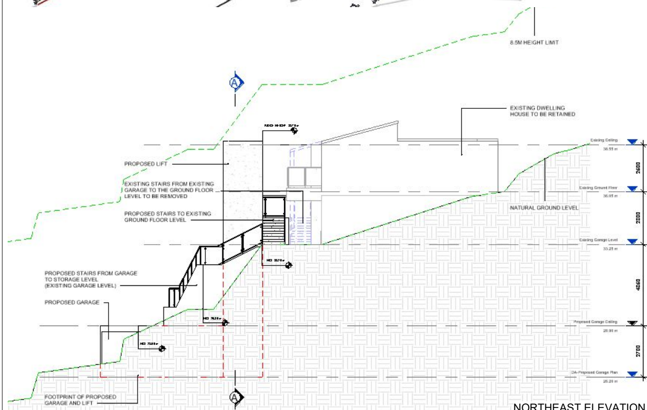
NORTHEAST ELEVATION
