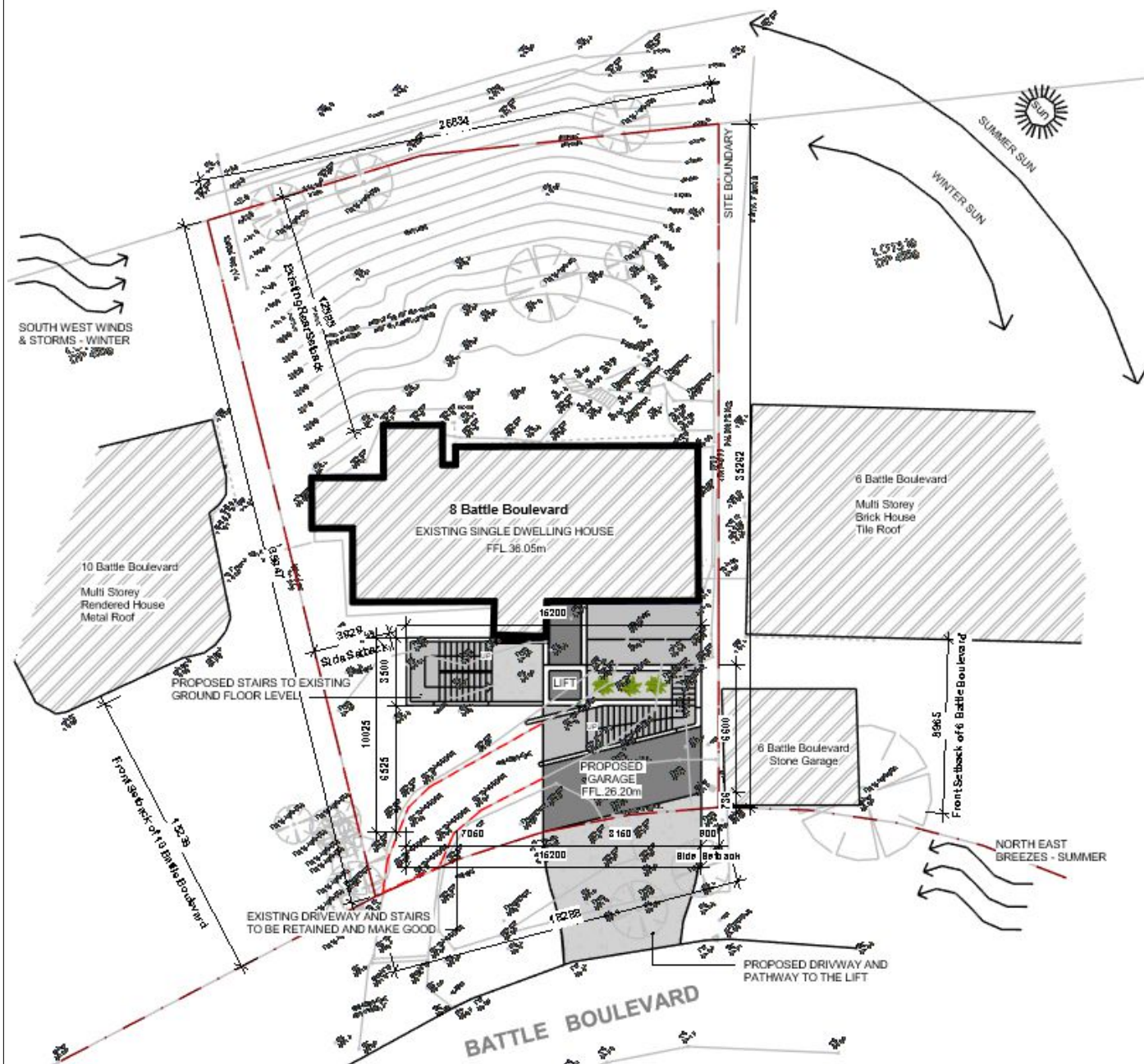
SITE PLAN
