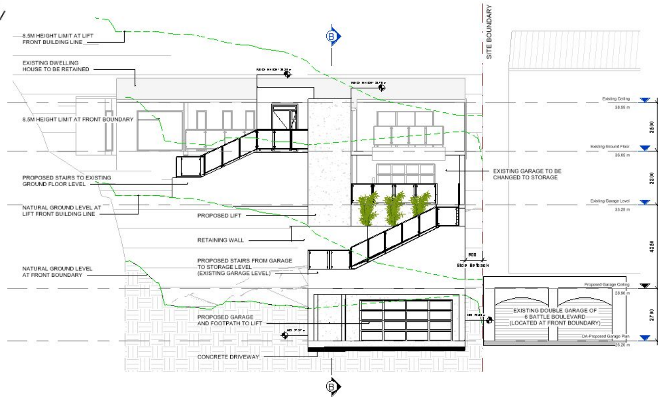
SOUTHEAST ELEVATION
