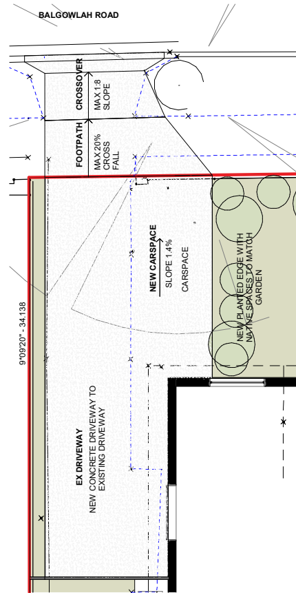
1 Proposed plan 1 : 100 REF:1/A3005
