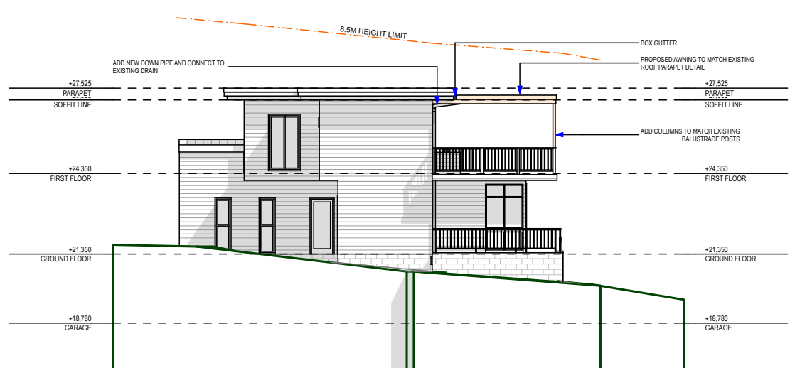
EAST ELEVATION
