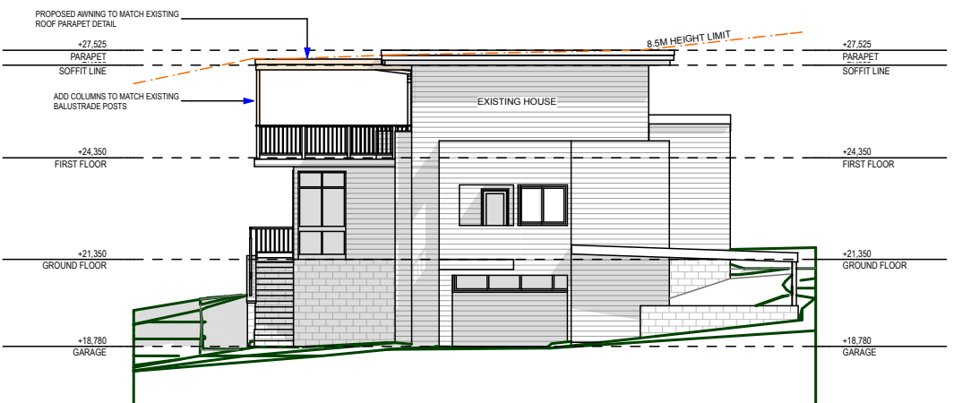
WEST ELEVATION
