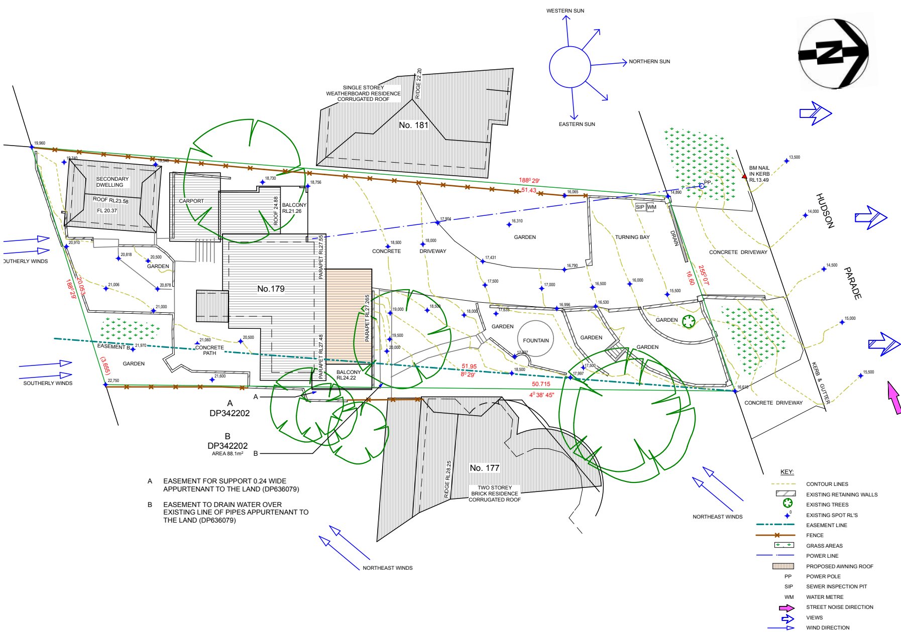
SITE PLAN
