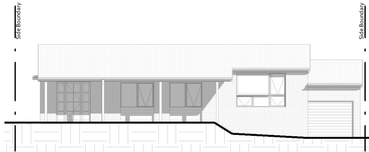
North Elevation
