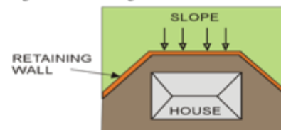
Fig. 10 Soil Drainage Plan
