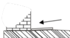
Fig. 20 Adjoining property water flows
