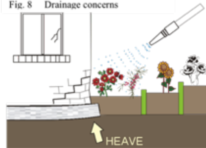
Fig. 8 Drainage concerns
