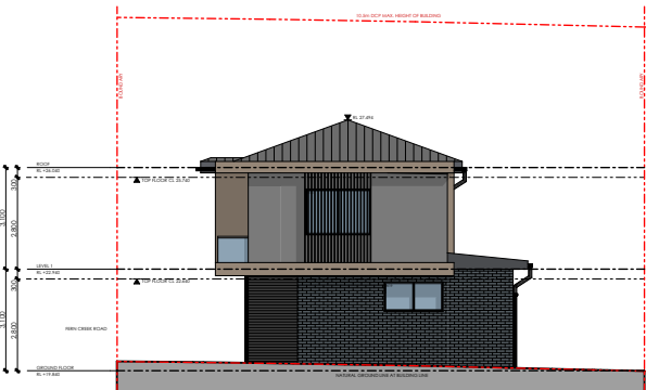
SOUTH ELEVATION 1:250
