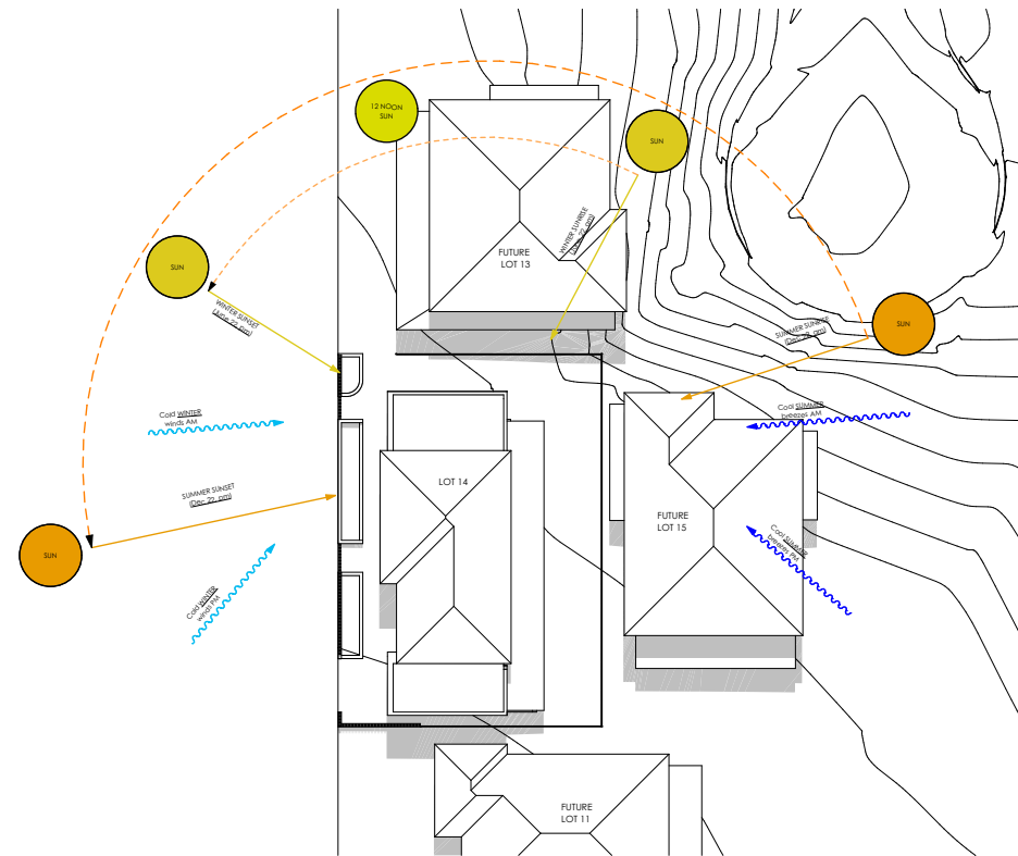
SITE ANALYSIS PLAN 1:500
