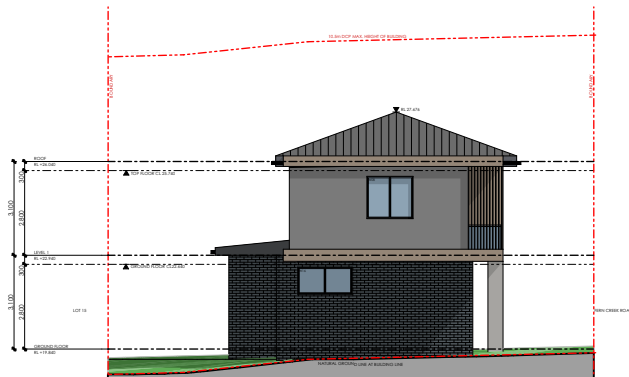
NORTH ELEVATION 1:250
