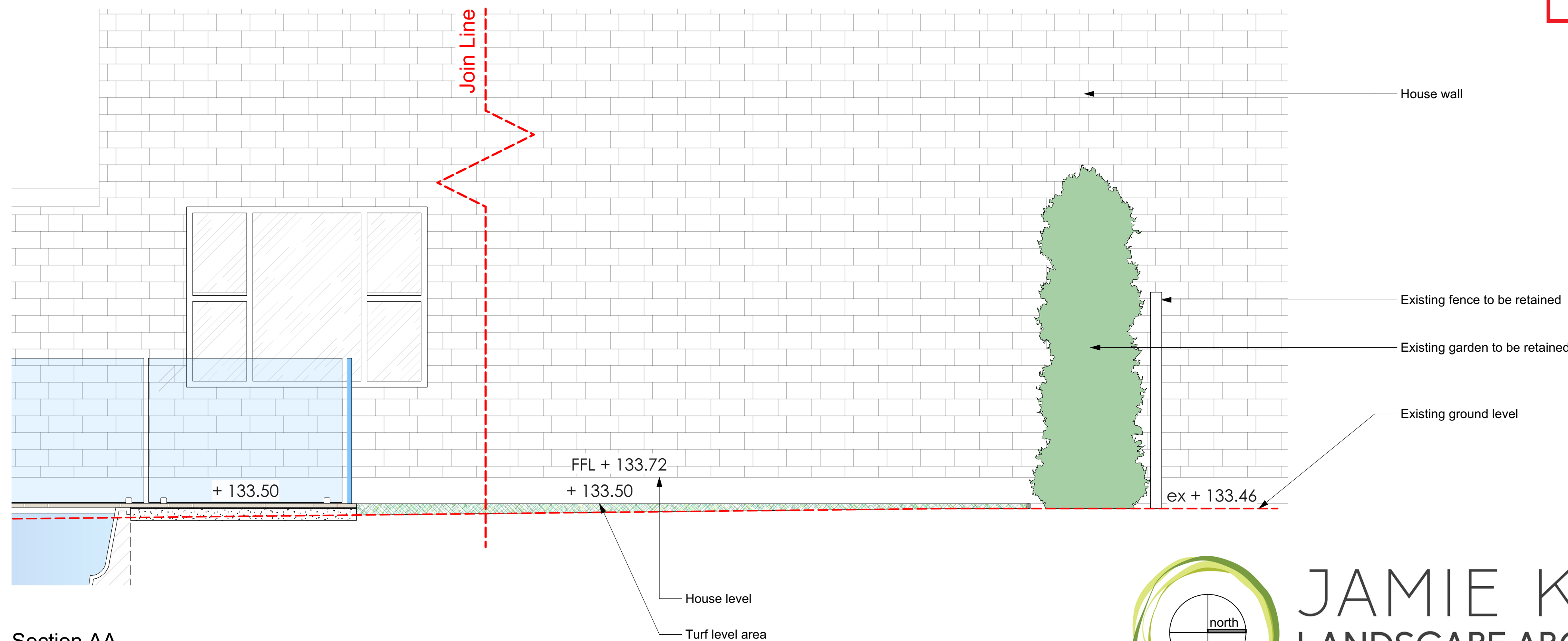
Section AA 1:25@A1 1:50@A3. Do not scale off plan
