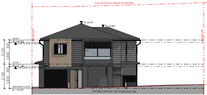
1 WEST ELEVATION 1:250
