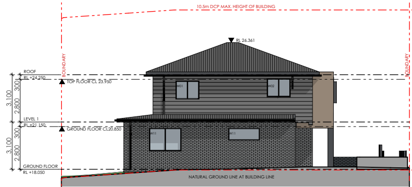
3 NORTH ELEVATION 1:250
