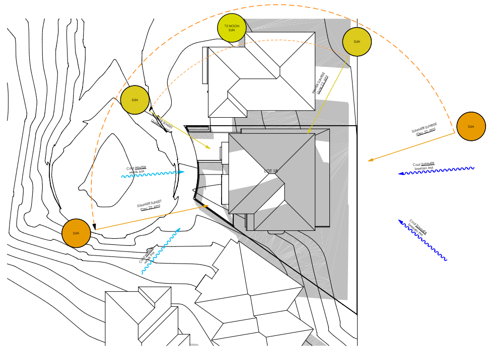
5 SITE PLAN / SITE ANALYSIS 1:500
