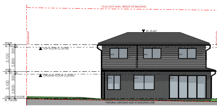
2 EAST ELEVATION 1:250
