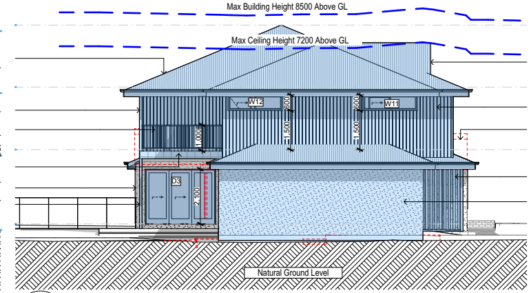
East 1:200
