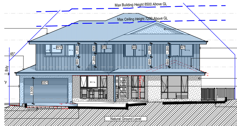
North 1:200
