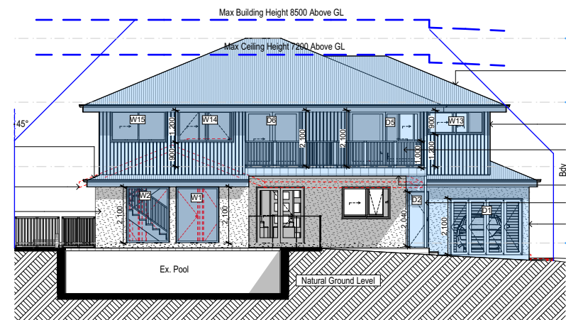
South 1:200
