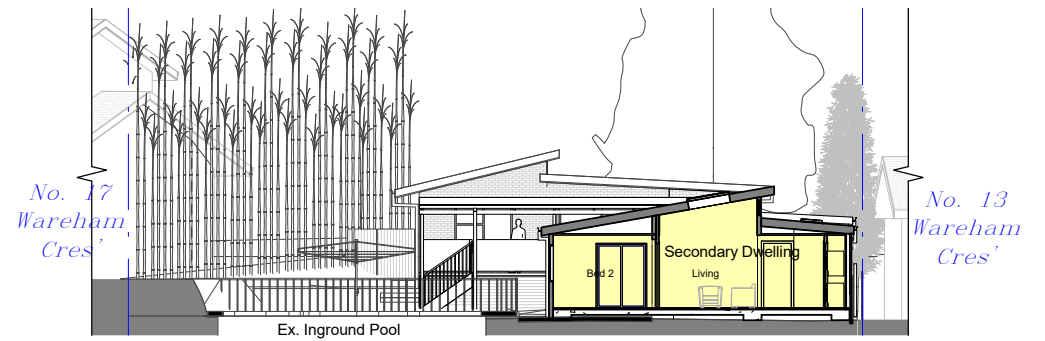
East Elevation 1:250
