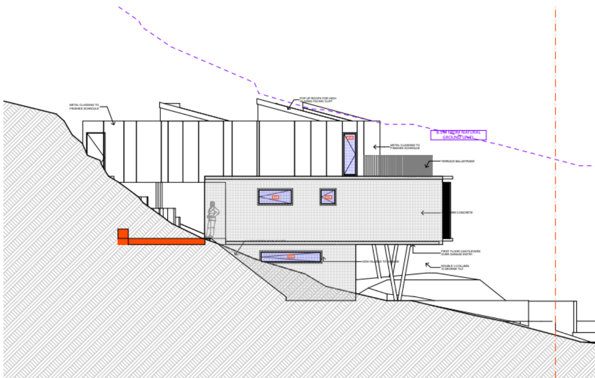
Figure 4: Side elevation.
