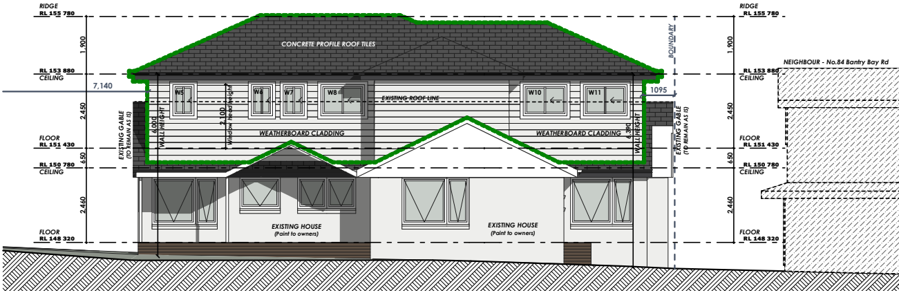
WEST ELEVATION (REAR ELEVATION)
