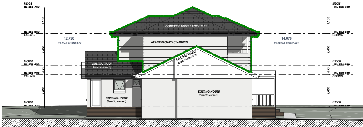
SOUTH ELEVATION
