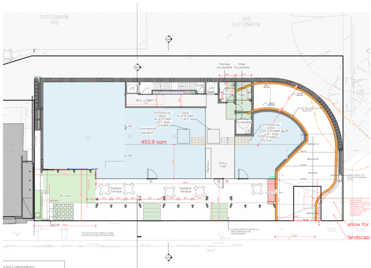
Figure 3.2 – Proposed Ground Floor Plan (Rob Mills Architects, 2021)
