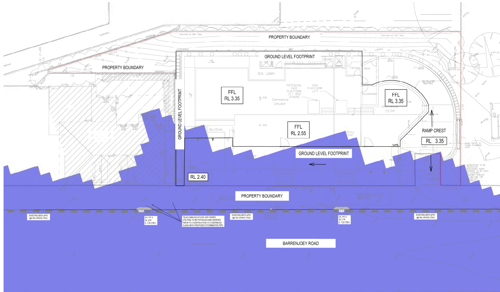
Figure 4.3 – Probable Maximum Flood Extents (Northern Beaches Council, 2021)
