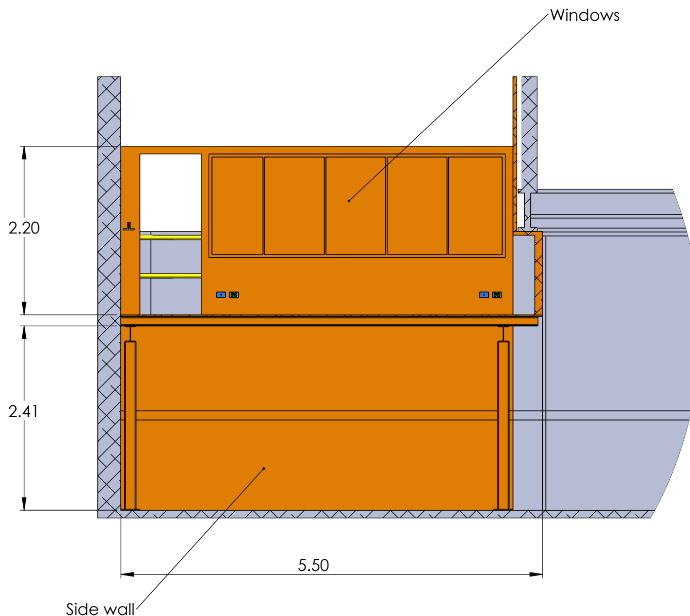
DETAIL N SCALE 1 : 50
