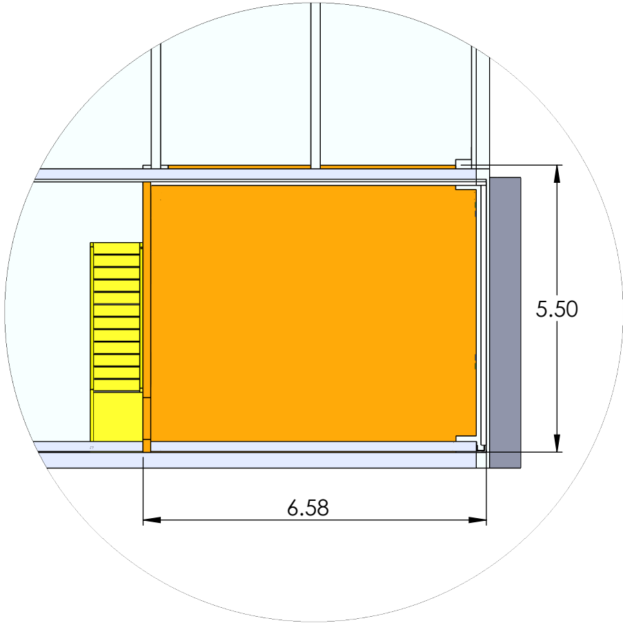
DETAIL E SOUTH MEZZANINE SCALE 1 : 100
