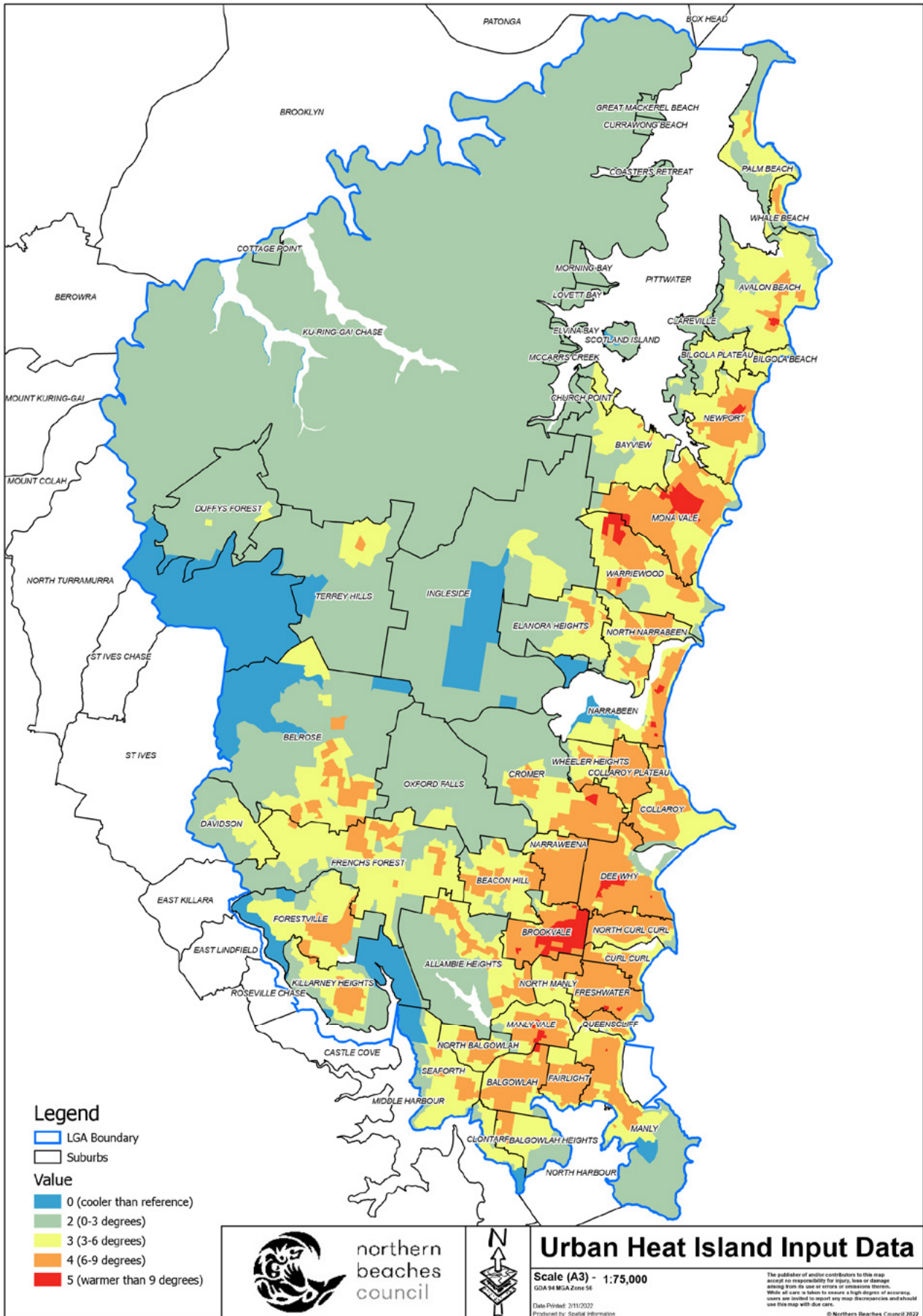
Urban Heat Island (UHI) effect across the suburbs of Northern Beaches
