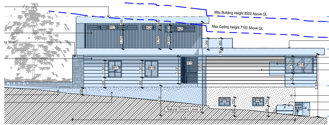
E-02 East 1:200
