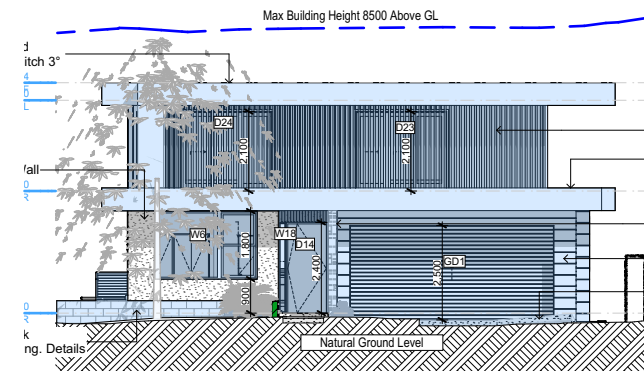
E-03 South 1:200
