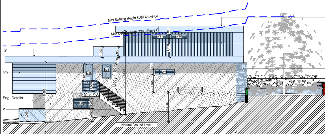
E-04 West 1:200
