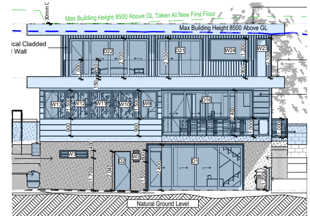
E-01 North 1:200
