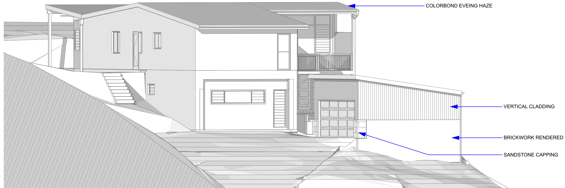
FRONT VIEW
