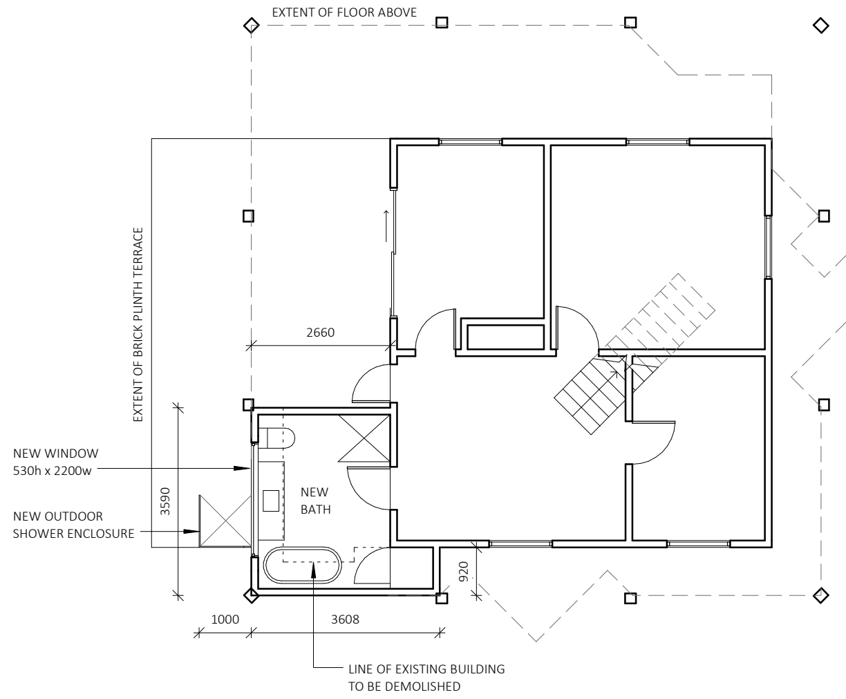
2 LEVEL 1 PROPOSED 1 : 100
