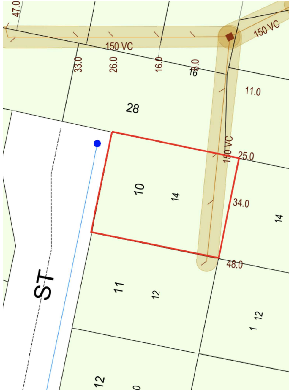
SERVICE LOCATION PRINT NOT TO SCALE
