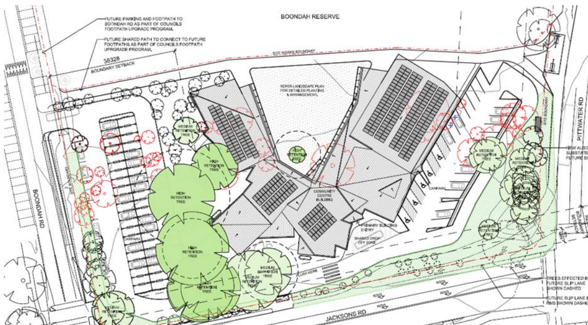
Figure 2 – Site Plan extract showing the proposed works within the site (source: Terroir Architects)
