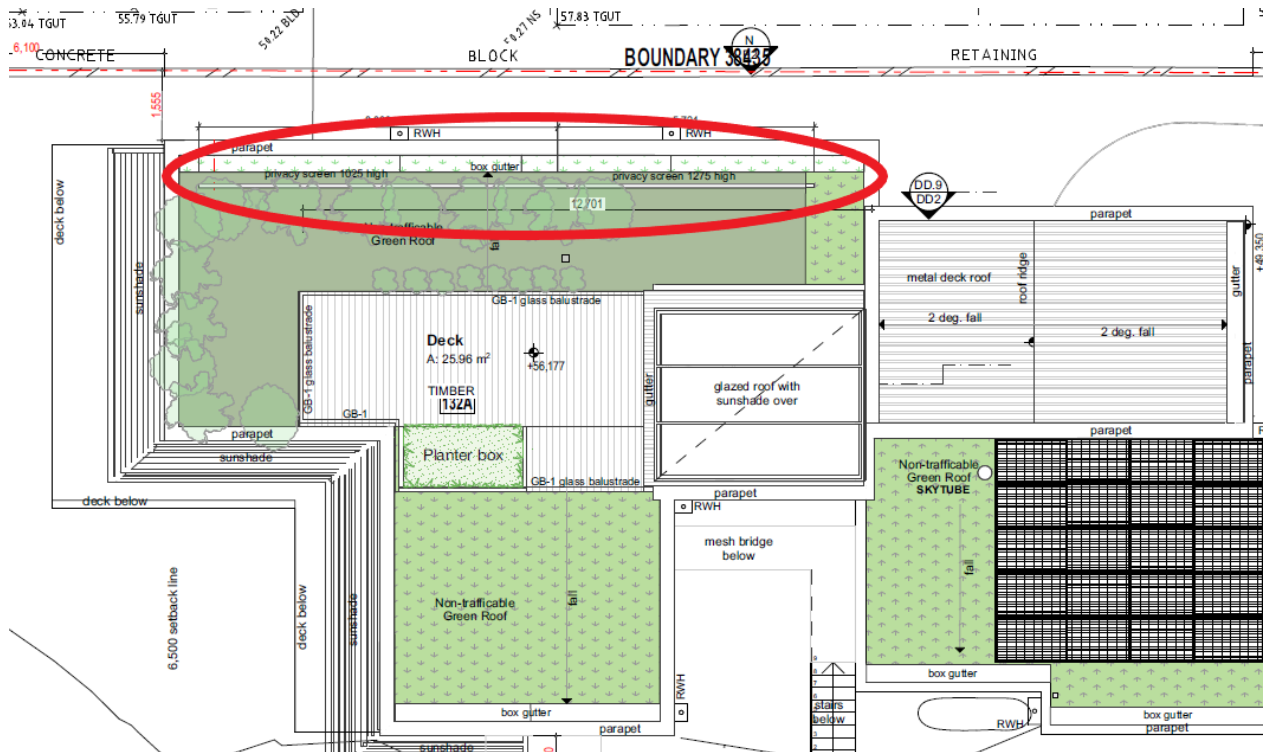
Figure 2: Privacy screen
