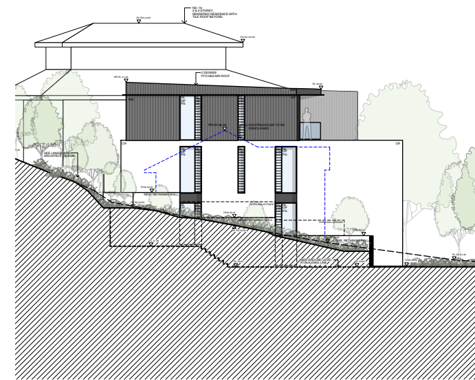
North Elevation 1:300
