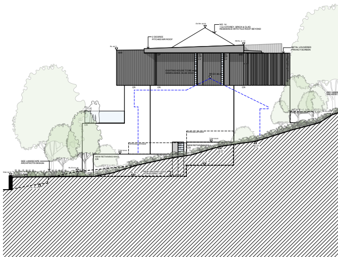
South Elevation 1:300
