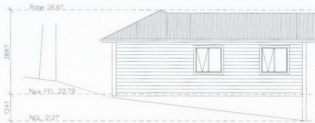
SOUTH ELEVATION
