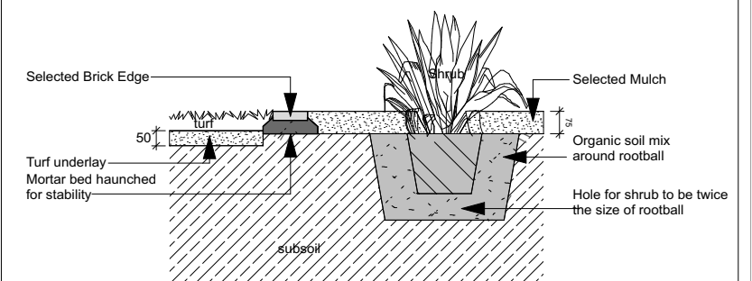
Typical Planting / Brick Edge Detail NOT TO SCALE
