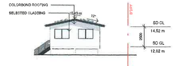
3 SD - SW ELEVATION.
