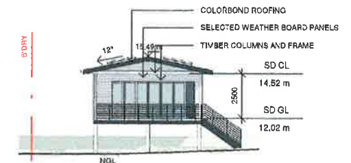
2 SD - NE ELEVATION.
