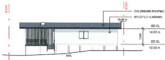
4 SD - NW ELEVATION.
