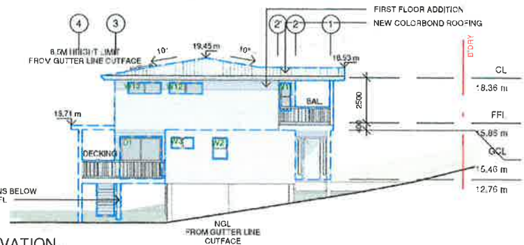
5 NE ELEVATION.
