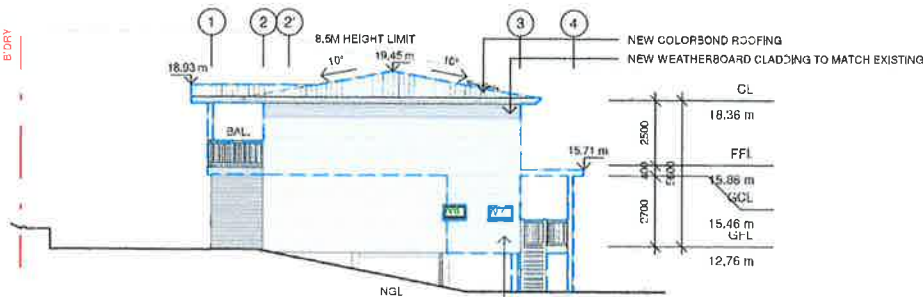
4 SW ELEVATION.
