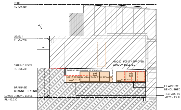
2 LONG COURTYARD 1:200
