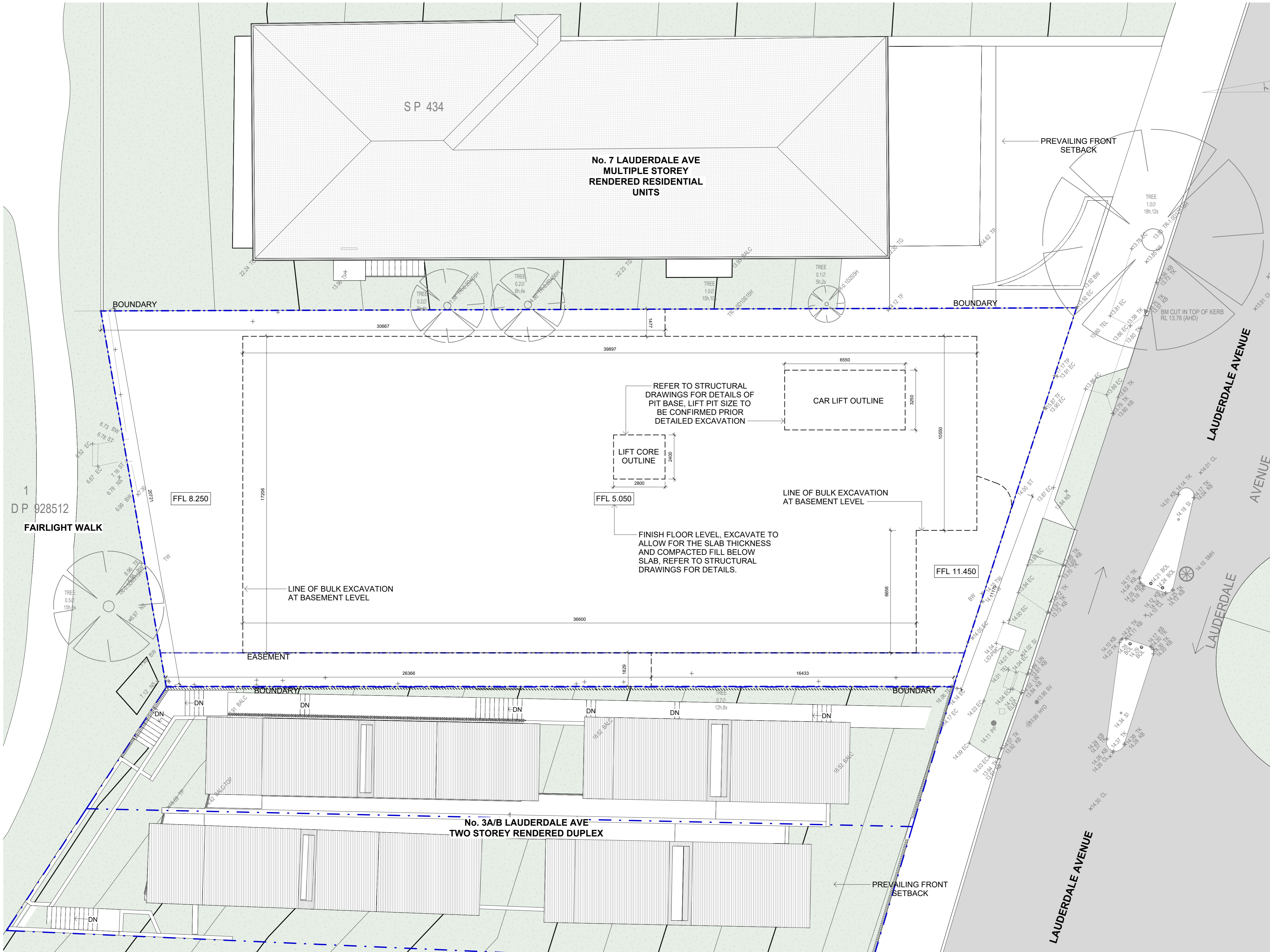
1 Excavation Plan 1:100
