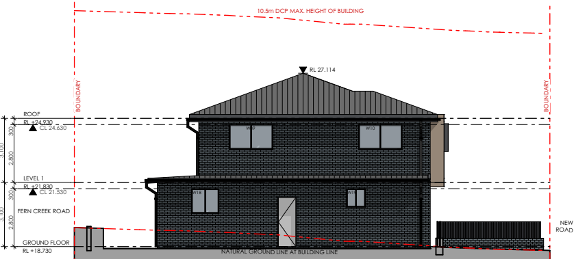
4 SOUTH ELEVATION 1:250
