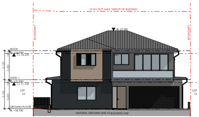
1 EAST ELEVATION 1:250
