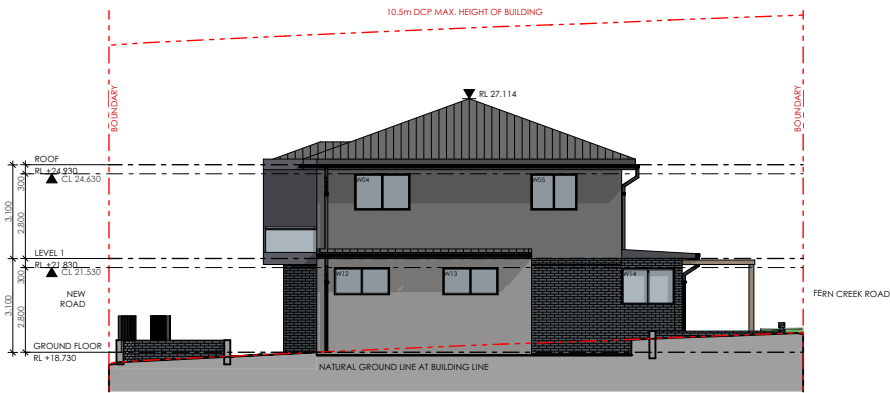
3 NORTH ELEVATION 1:250
