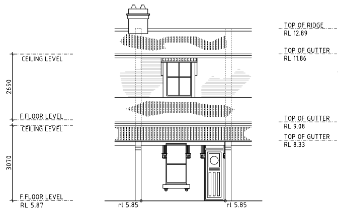
EAST ELEVATION
