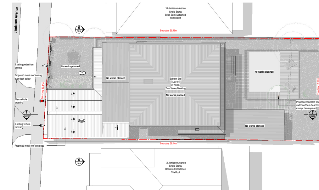
1 Proposed Site Plan 1:100
