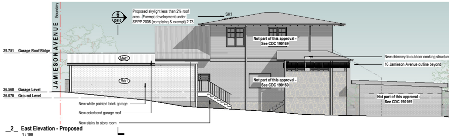
2 East Elevation - Proposed 1:100
