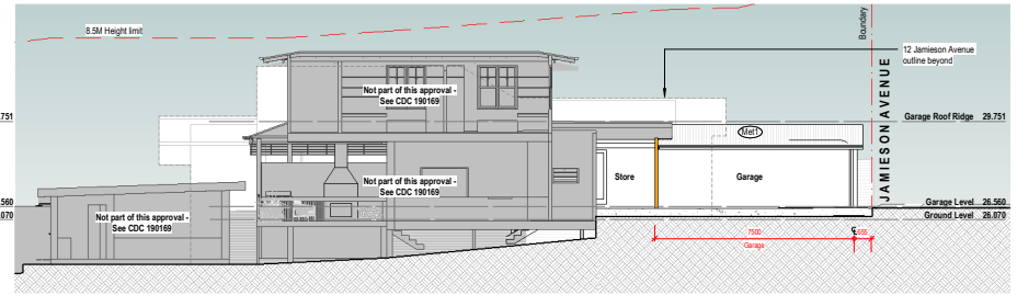
7 Section - Proposed 1:100
