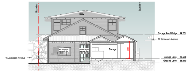
6 Section - Proposed 1:100
