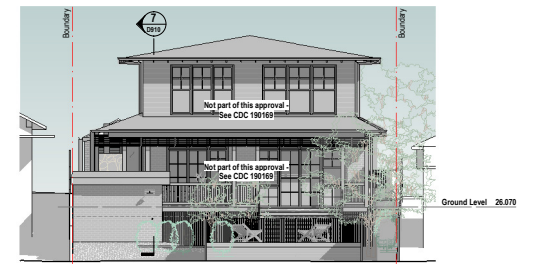
4 North Elevation - Proposed 1:100
