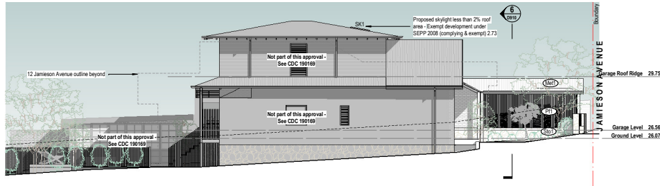
3 West Elevation - Proposed 1:100
