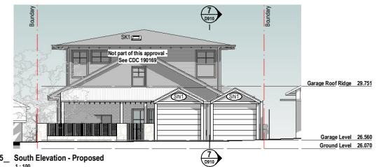
5 South Elevation - Proposed 1:100
